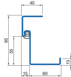
Blockzarge 95 / 75 mm
