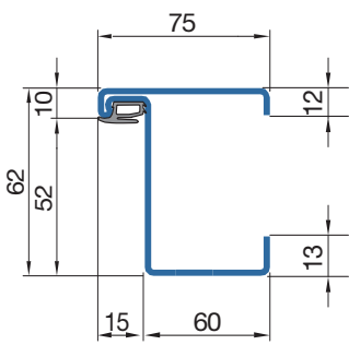
Blockzarge 62 / 75 mm
