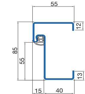
Blockzarge 95 / 55 mm
