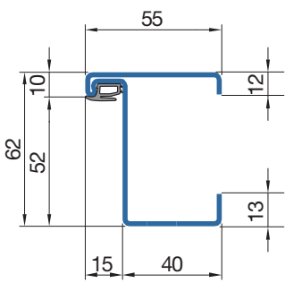
Blockzarge 62 / 55 mm
