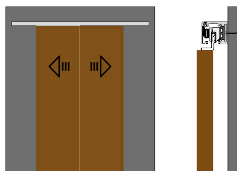
Wandmontage
