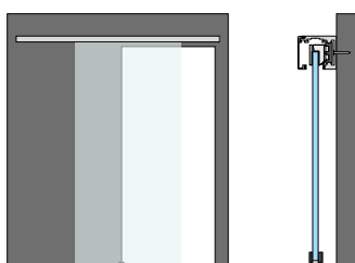
Wandmontage
